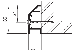
+1' Fixing 'A' Frame
