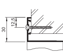
+1' Fixing 'S' Frame
